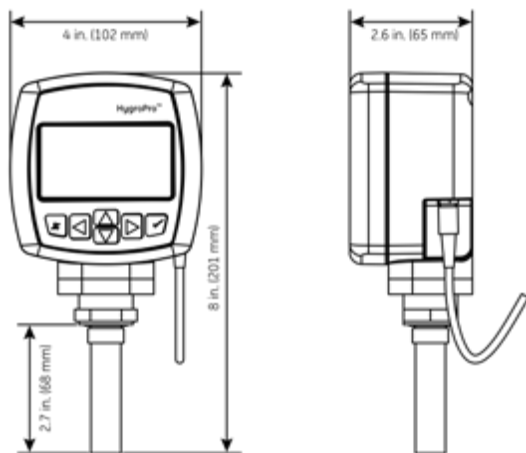
HygroPro dimensions
