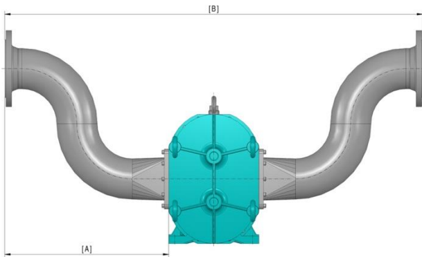
Design 6 | Gooseneck version in mm / inches (approx.)
