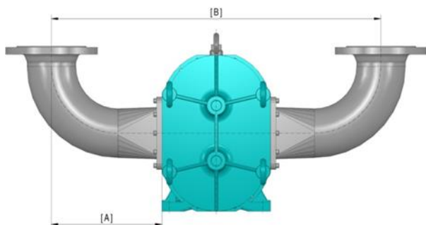
Design 2 | 90° elbow up in mm / inches (approx.)
